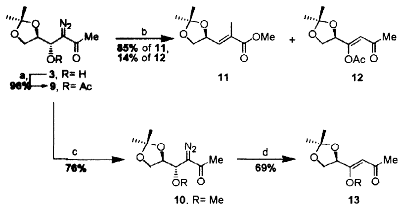
Scheme 2. Reagents and Conditions. (a) 2.0 equiv of Ac 2 O, pyr, 25 °C, 8 h, 96%. (b) hv (λ = 253.7 nm), MeOH:THF (1:9), -30 °C, 17 h, 85% of 11, 14% of 12. (c) 4.0 equiv of MeI, 2.0 equiv of NaOH (powder), DMF, 25 °C, 24 h, 76%. (d) hv (λ = 253.7 nm), MeOH:THF (1:9), 4 °C, 10 h, 69%.
