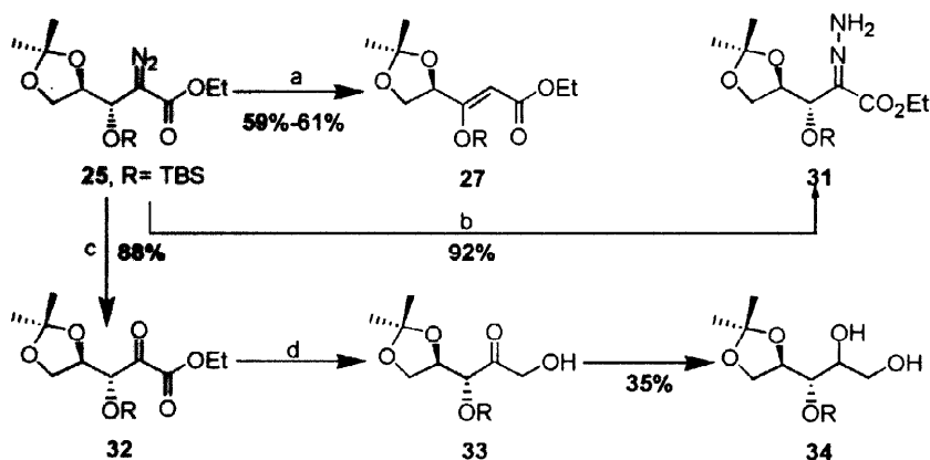
Scheme 6. Reagents and Conditions. (a) 1.1 equiv of \text{Me}_3\text{Al} (2 M in toluene), toluene, -78^\circ\text{C} \rightarrow 0^\circ\text{C} , 2 h, 59% or 1.1 equiv of \text{Et}_2\text{Zn} (1 M in toluene), toluene, -78^\circ\text{C} \rightarrow 0^\circ\text{C} , 2 h, 61%. (b) 3.0 equiv of \text{LiHEt}_3\text{B} (1 M in THF), THF, 0^\circ\text{C} , 1 h, 92%. (c) 1.5 equiv of m CPBA, \text{CH}_2\text{Cl}_2 , 0^\circ\text{C} , 6 h, 88%. (d) 4.0 equiv of \text{NaBH}_4 , \text{MeOH} , 0^\circ\text{C} , 0.5 h, 35%.
