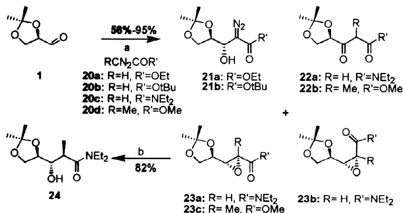
Scheme 4. Reagents and Conditions. (a) i. 1.5 equiv of 20a , neat, 4 °C, 12 h, 68% of 21a . ii. 1.5 equiv of 20b , neat, 4 °C, 12 h, 70% of 21b . iii. 1.5 equiv of 20c , neat, 25 °C, 12 h, 12% of 22a , 18% of 23a , 28% of 23b . iv. 1.5 equiv of 20c , CHCl 3 , 25 °C, 12 h, 40% of 23a , 45% of 23b . v. 1.5 equiv of 20d , neat, 4 °C, 12 h, 68% of 22b , 23% of 23c . (b) 1.5 equiv of Me 2 CuLi, diethyl ether, -10 °C, 2 h, 82%.
