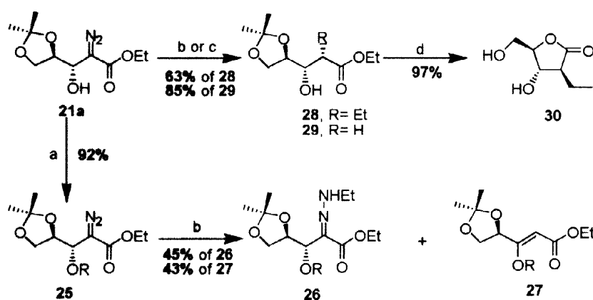
Scheme 5. Reagents and Conditions. (a) 1.5 equiv of TBSCl, 2.0 equiv of imidazole, DMF, 25 °C, 12 h, 92% (b) 1.2 equiv of Et 3 B (1 M in THF), THF, 25 °C, 12 h, 45% of 26 , 43% of 27 , 63% of 28 . (c) 1.5 equiv of 9-BBN (0.5 M in THF), THF, 25 °C, 6 h, 85% (d) 20% TFA in EtOH, EtOH-H 2 O, 0 °C, 5 h, 97%.
