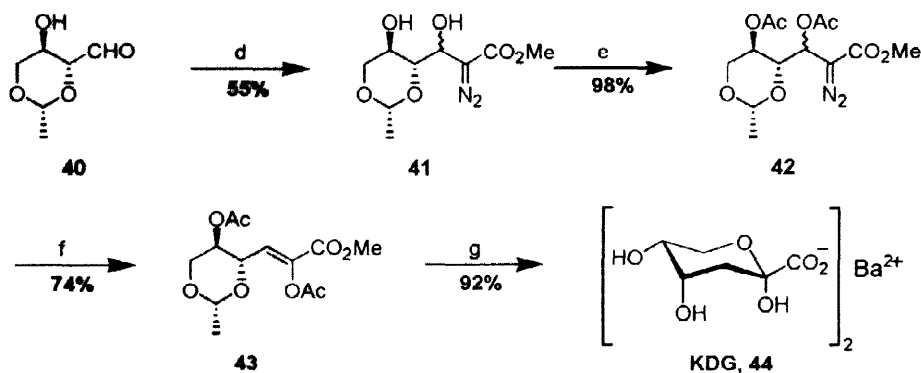
Scheme 7. Reagents and Conditions. (a) 2.0 equiv of \text{Ac}_2\text{O} , pyr, 25 °C, 5 h, 98%. (b) 2. = equiv of \text{O}[\text{OCO}_2\text{tBu}]_2 , pyr, 25 °C, 12 h, 98%. (c) \text{Rh}_2(\text{OAc})_4 (catalytic), \text{CHCl}_3 , 25 °C, 0.5 h, 97%. (d) 2.0 equiv of \text{HCN}_2\text{CO}_2\text{Me} , 0.5 equiv of KOH (10% solution in MeOH), MeOH, 25 °C, 1 h, 55%. (e) 2.0 equiv of \text{Ac}_2\text{O} , pyr, 25 °C, 5 h, 98%. (f) \text{Rh}_2(\text{OAc})_4 (catalytic), \text{CHCl}_3 , 25 °C, 0.5 h, 74%. (g) 20 % TFA in MeOH, MeOH- \text{H}_2\text{O} , 60 °C, 8 h, then 3.0 equiv of \text{Ba}(\text{OH})_2 , MeOH- \text{H}_2\text{O} , 25 °C, 3 h, 92%.
