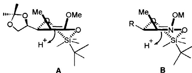
Figure 2. Intermediates Structures in the Stereoselective Protonation
