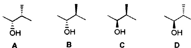
Figure 1. Fragments of Macrolide Type Antibiotics.
